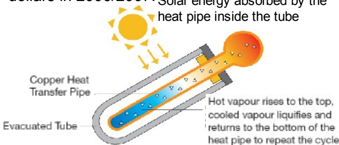
Figure 2 Hills Solar tube collector cross section
